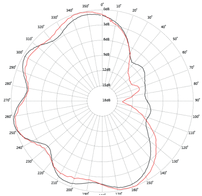
Simulated and measured antenna pattern
